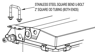
STAINLESS STEEL CEILING MOUNTING BRACKET (BOTH ENDS)
