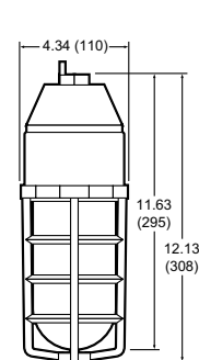
Pendant Fluorescent/HID
