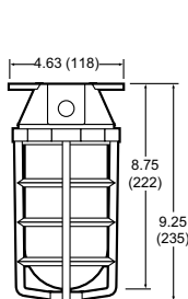
Ceiling Incandescent
