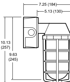
Wall Incandescent
