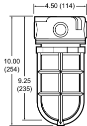
Ceiling Incandescent
