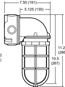
Wall Incandescent
